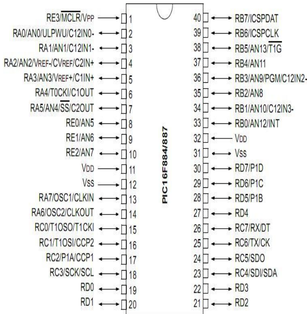
Figure10. Pin Configuration of PIC 16F887 Micro-controller
