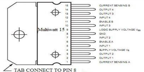
Fig11. Pin connection of L298 motor driver.
