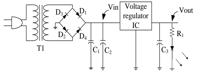
Figure7. Power Supply Circuit Diagram
