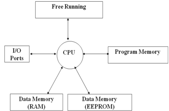
Fig 8. Block diagram of PIC microcontroller
