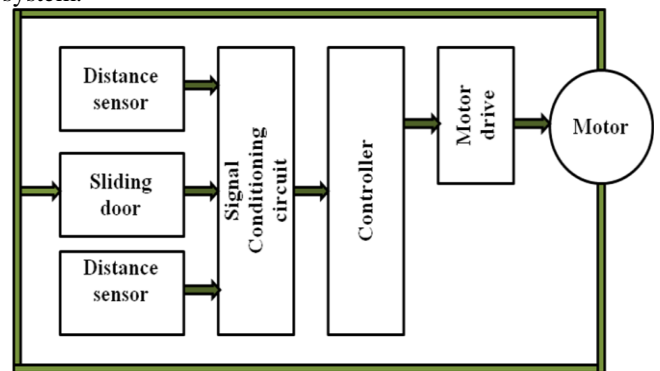
Fig9. Proposed block diagram of automatic control system of sliding door
