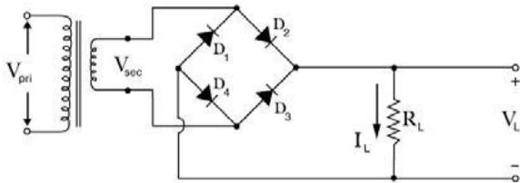
Fig 5. Full-wave bridge rectifier
