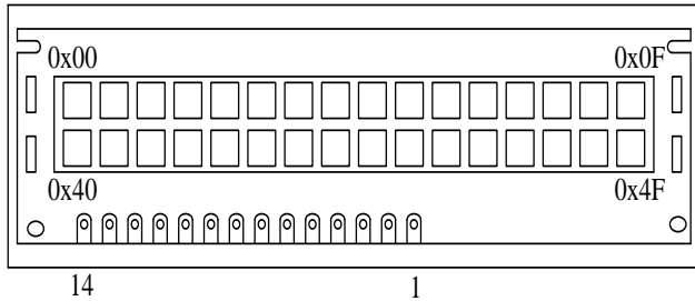
Fig12. LCD Display with 2 Lines x 16 Characters
