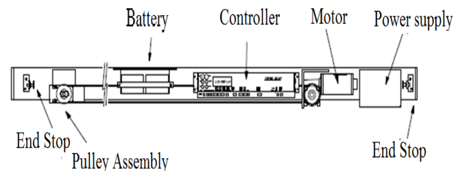
Fig1. Schematic Diagram of Automatic Sliding Door Operator
