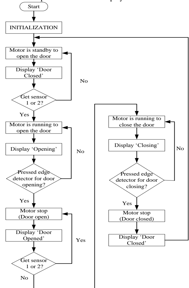
Figure 16.System Flow Chart
