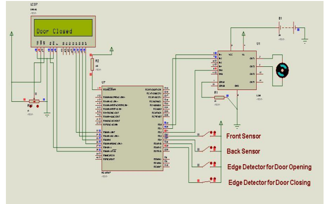
Fig22. Simulation circuit of automatic sliding door system
